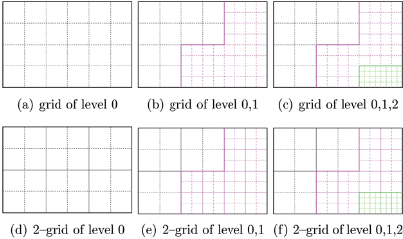
Fig. 1. – Grids and d -grids for d = 2 .
