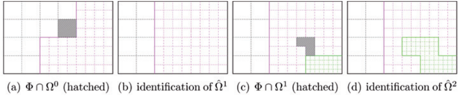
Fig. 2. – Identification of \hat{\Omega}^1 and \hat{\Omega}^2 in Example 1.
