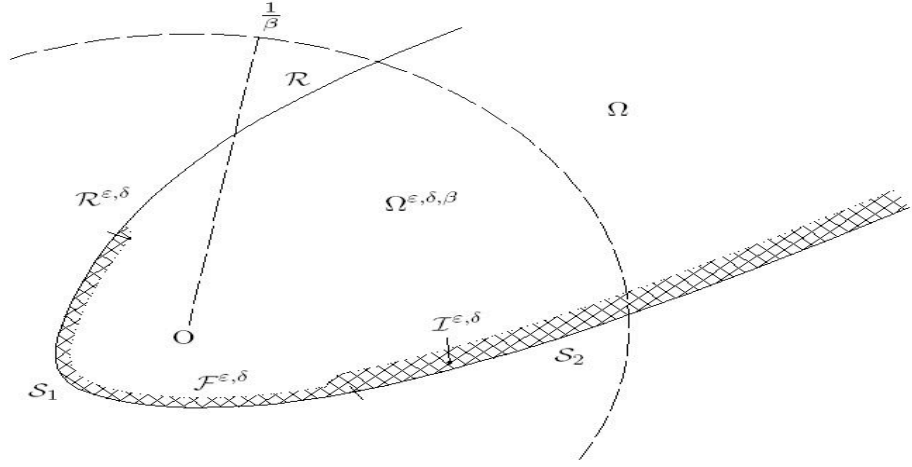
FIGURE 2. Unbounded \Omega .
