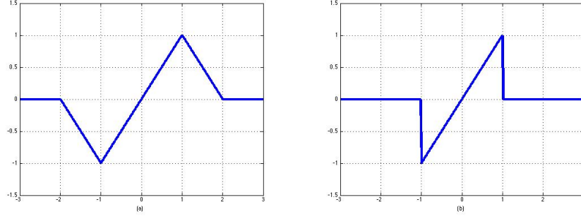
FIGURE 1.1: Froese and Oberman's filter (left), Oberman and Salvador's filter (right)
