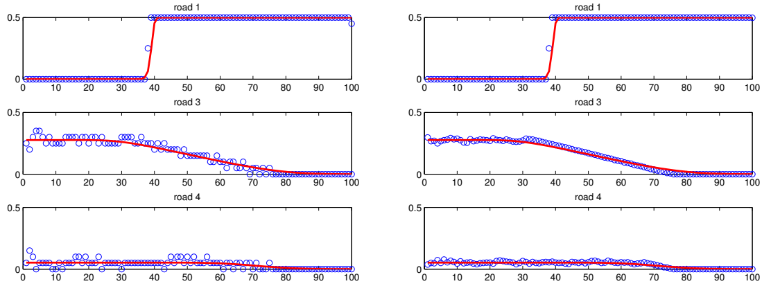
FIGURE 4.10: Diverge, results of the simulation at final time. Total density \omega^p redefined on roads (red line) and density of microscopic vehicles \Psi (blue circles). Left: \ell_n = 2 (max number of cars per cell = 20), \Delta t = 4 . Right: \ell_n = 0.1 (max number of cars per cell = 400), \Delta t = 0.25 .
