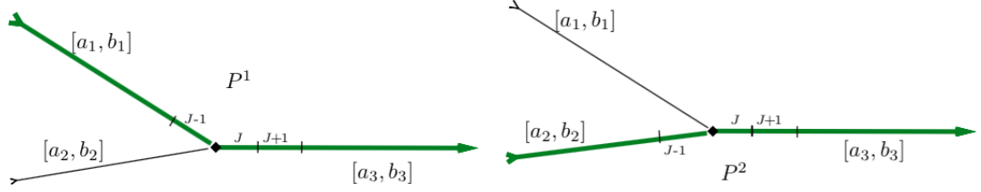
FIGURE 4.4: A network with 3 arcs and 1 junction, representing a merge. Path P^1 (left) and path P^2 (right).
