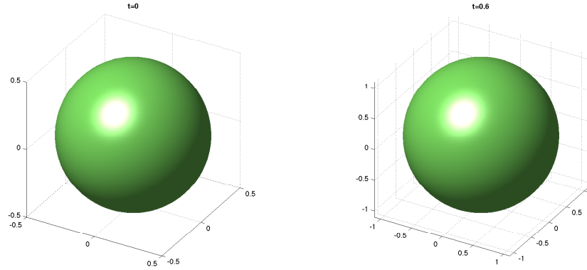
FIGURE 2.13: Example 2.3.7, plots at time T = 0 (left) and T = 0.6 (right) for the filtered scheme with mesh point M = N = P = 100 .
