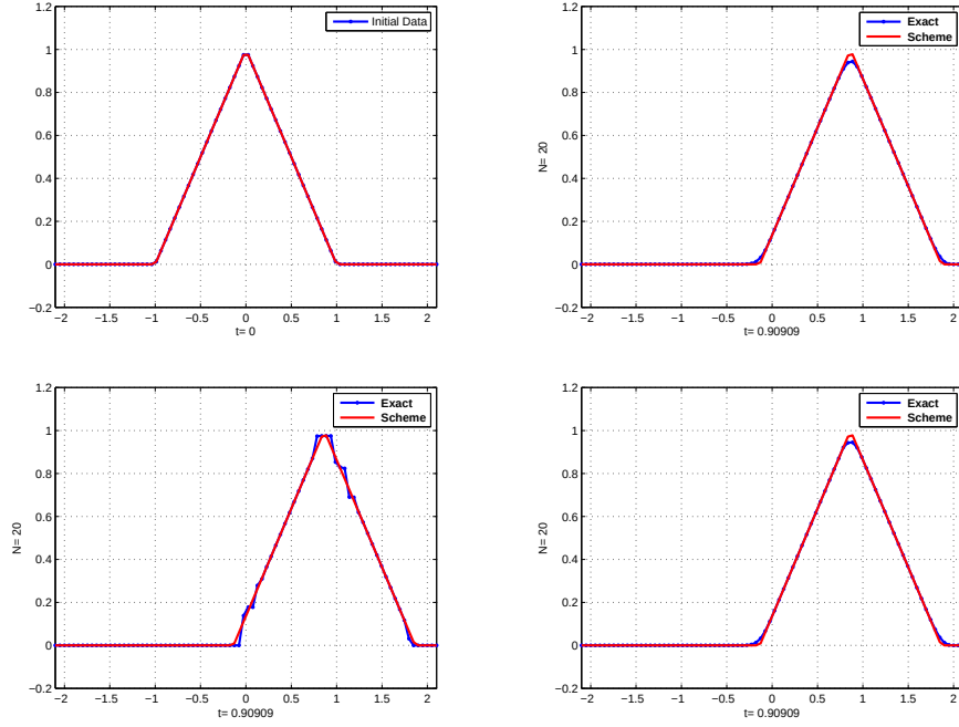
FIGURE 3.4: (Example 3.5.1), on the top left is the plot of initial data (3.49) and on top right SL- P^1 scheme. In the second row plot of Ultrabee and coupled scheme at t = 20\Delta t where \Delta t = 0.045 .
