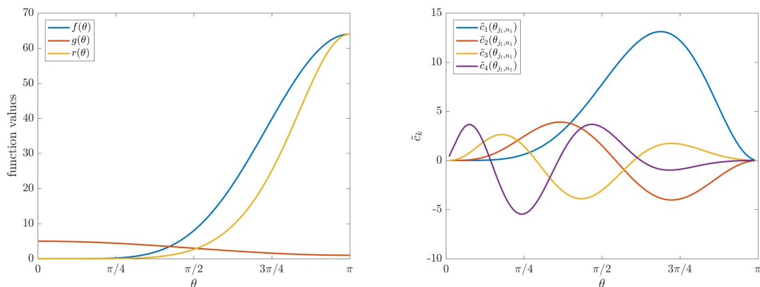
Figure III.2: Example 2: Generating functions ( f , g , and r ) and \tilde{c}_k for k = 1, 2, 3, 4 .
