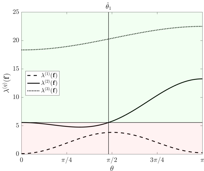
Figure V.9: Example 3: The three eigenvalue functions, \lambda^{(q)}(\mathbf{f}) , q = 1, 2, 3 .
