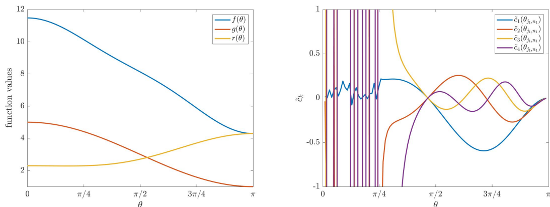
Figure III.5: Example 5: Generating functions ( f , g , and r ) and \tilde{c}_k for k = 1, 2, 3, 4 .
