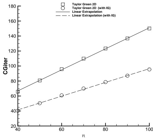
(a) k = 2
