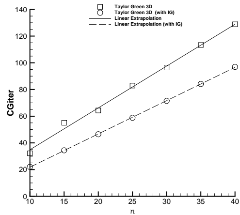
(b) k = 3
