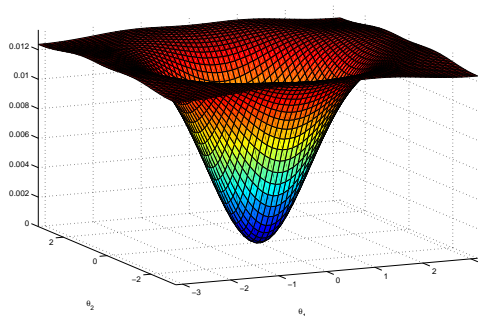
Figure II.8: \det \mathbf{f}(\theta_1, \theta_2) , (\theta_1, \theta_2) \in \mathcal{I}_2
