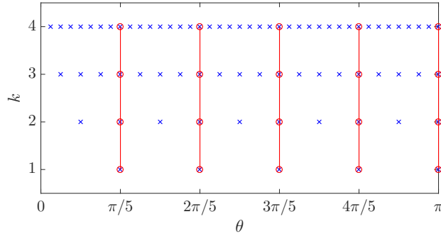
Figure IV.3: Representation of the grids \theta_{[n_k]} , k = 1, \dots, \alpha , for n_1 = 5 and \alpha = 4 . Red circles represent the grid points \theta_{j_k, n_k} and blue x's represent the rest of the grid points of \theta_{[n_k]} .
