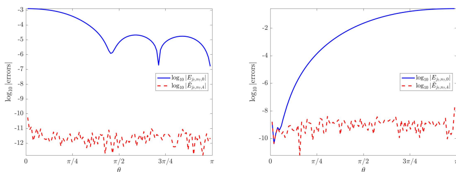
Figure III.12: Example 3 and 4: The errors \log_{10} |E_{j_7, n_7, 0}| and \log_{10} |\tilde{E}_{j_7, n_7, 4}| for the 100 indices j_7 of n_7 = 6463 in (III.19), corresponding to n_1 = 100 , and using \tilde{c}_k, k = 1, 2, 3, 4 , computed with \gamma = 2 .
