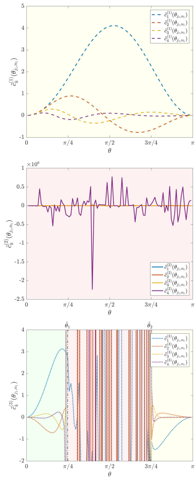
Figure V.7: Example 2: Computations made with n_1 = 100 , \alpha = 4 . From the top to the bottom panel the approximations \hat{c}_k^{(q)}(\theta_{j_1, n_1}) for \lambda^{(q)}(\mathbf{f}) , q = 1, 2, 3 .
